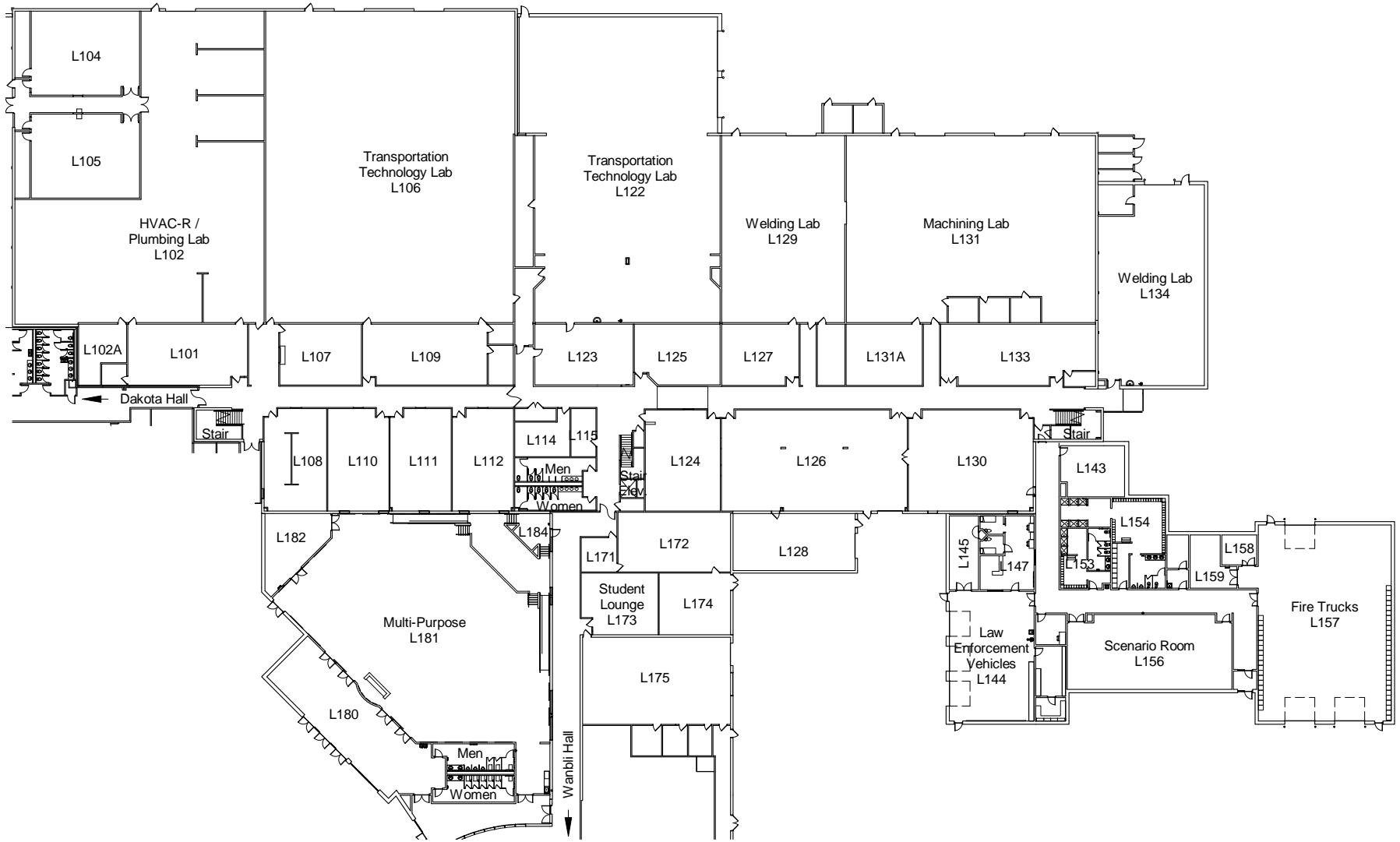
③ Lewis & Clark Hall - Level 1 1" = 60'-0"
