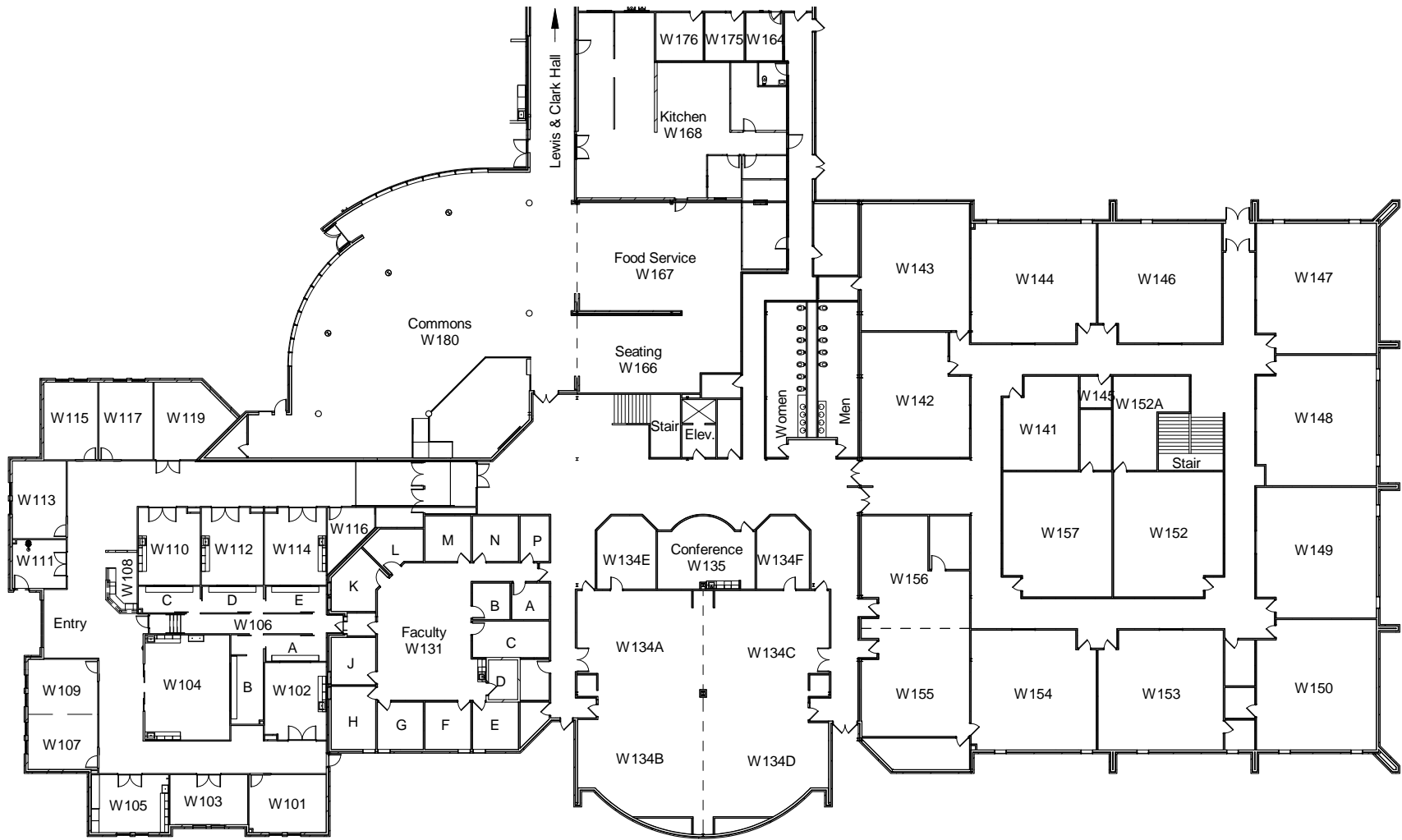
5 Wanbli Hall - Level 1 1" = 40'-0"
